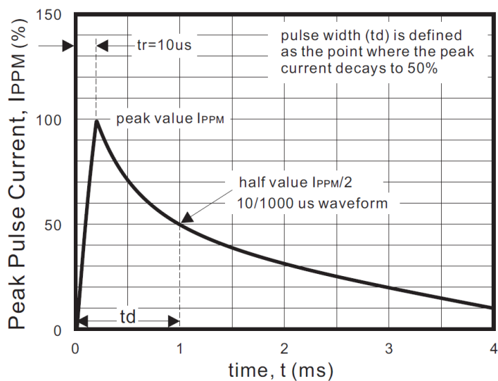
Fig3. PULSE WAVEFORM
