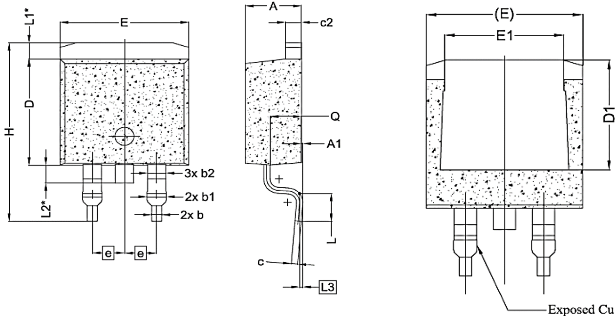
TO-263, 3 Leads
