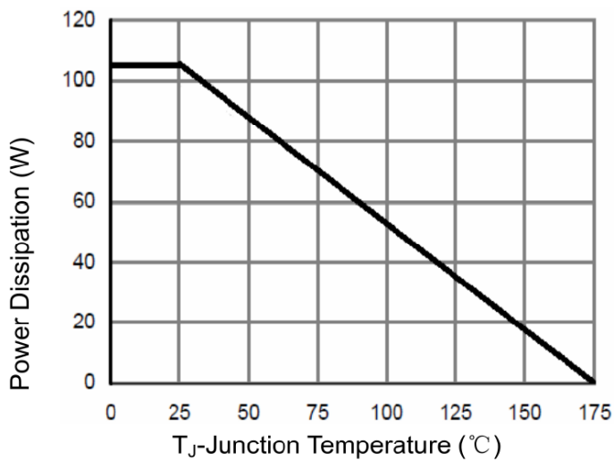
Fig.9 POWER DE-RATING
