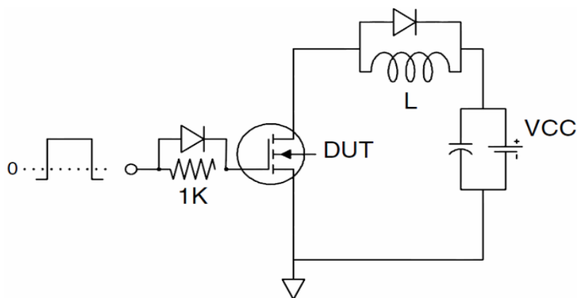
2) GATE CHARGE TEST CIRCUIT
