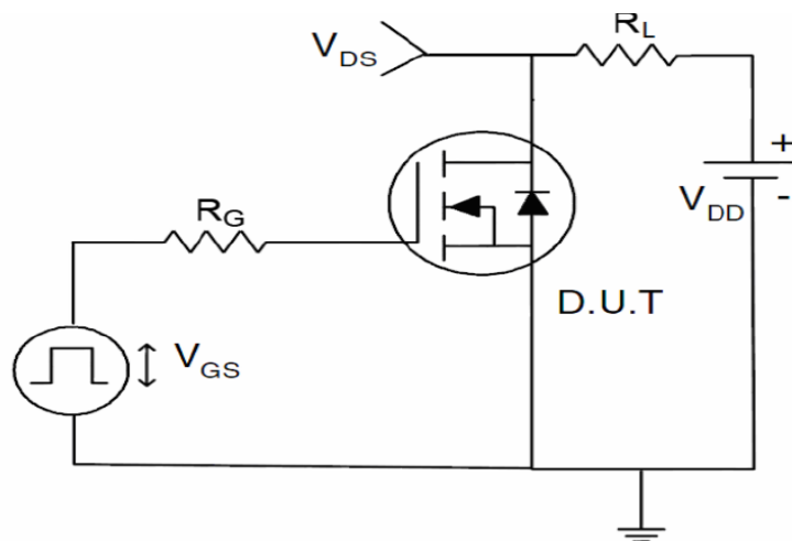
3) SWITCH TIME TEST CIRCUIT
