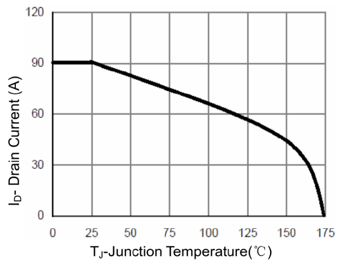
Fig.10 ID CURRENT DERATING
