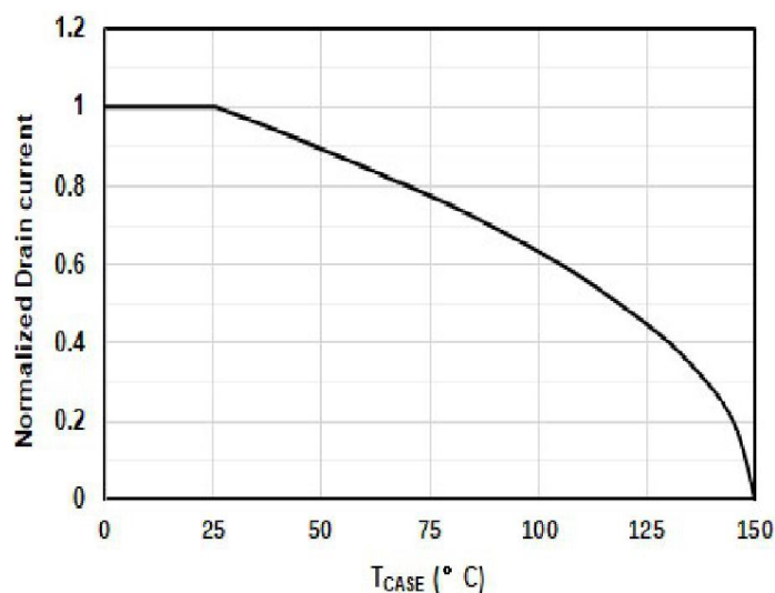
Fig.8 DRAIN CURRENT Vs. CASE TEMPERATURE
