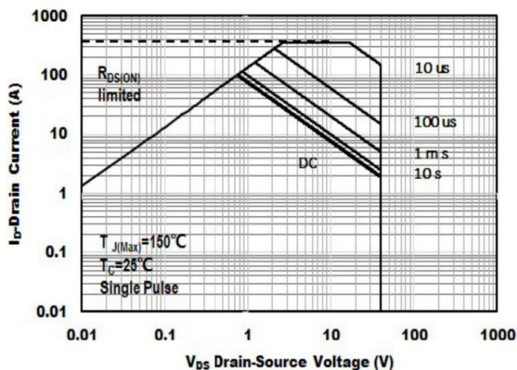
Fig.7 SAFE OPERATING AREA
