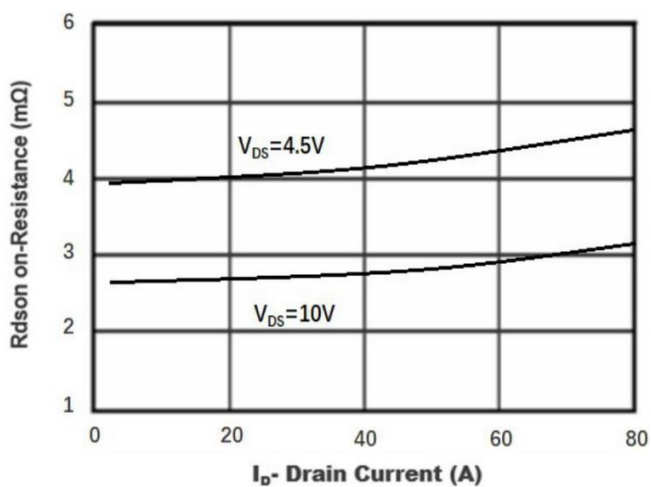
Fig.5 DRAIN-SOURCE ON RESISTANCE
