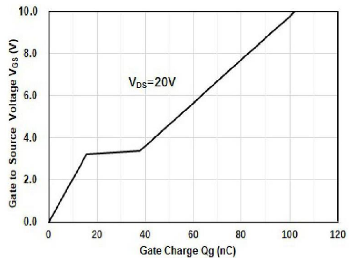
Fig.4 GATE CHARGE
